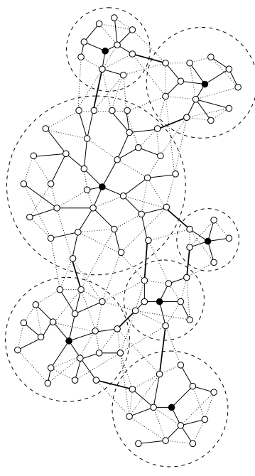
Figure 10.1: A cluster partition of a network: The dashed cycles specify the clusters, cluster leaders are black, the solid edges are the edges of the intracluster trees, and the bold solid edges are the intercluster edges
