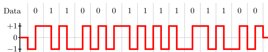
Figure 5.41: Manchester coding.
