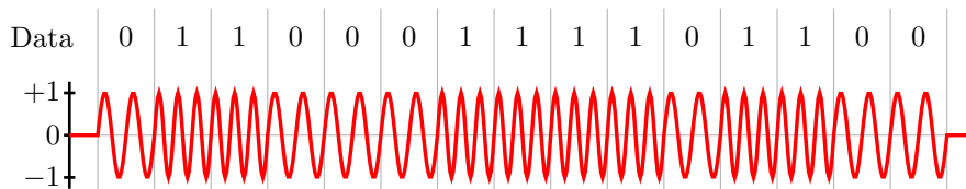
Figure 5.46: Frequency modulation.
