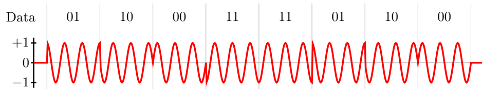
Figure 5.48: Phase modulation with 2-bit symbols.
