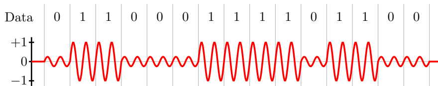
Figure 5.44: Amplitude modulation.
