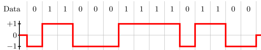
Figure 5.39: Simple line coding.
