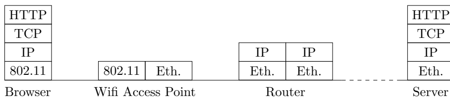
Figure 4.26: The browser issues an HTTP request over Wifi (802.11 link layer protocol) which is received by an access point and forwarded over Ethernet to a router. The router reads the IP header to identify the next hop and forwards the packet accordingly. Only the server needs to parse the entire stack of layers to get the original HTTP request.
