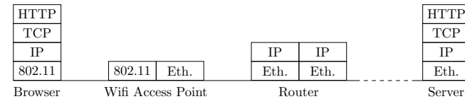
Figure 4.26: The browser issues an HTTP request over Wifi (802.11 link layer protocol) which is received by an access point and forwarded over Ethernet to a router. The router reads the IP header to identify the next hop and forwards the packet accordingly. Only the server needs to parse the entire stack of layers to get the original HTTP request.
