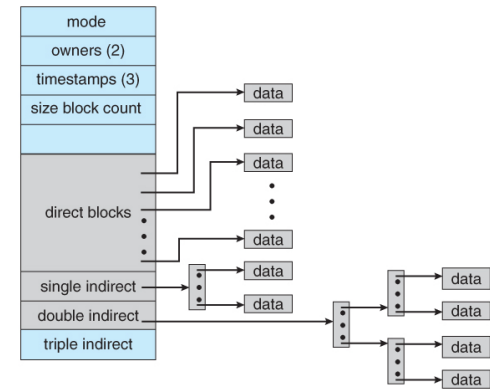
Figure 6.21: The structure of an inode. Direct pointers to blocks are referred to as “direct blocks” here. The inode in this example does not have a triple indirect pointer.
