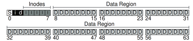
Figure 6.23: A high level view of how the file system is arranged on the storage device. S is the superblock, i the inode bitmap, d the data bitmap, I the inode region, and D the data region. The numbers refer to blocks. i is usually smaller than d .
