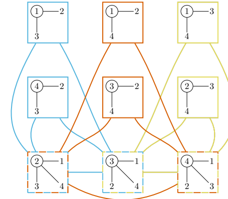
Figure 5.8: 1-neighborhood graph \mathcal{N}_1(\mathcal{G}) of the family in Figure 5.7. The colors of 1-hop views indicate which graphs in \mathcal{G} they can be found in. The colors of edges indicate which graphs in \mathcal{G} contain neighboring nodes that have the connected 1-hop views.
