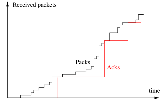
Figure 2: TCP ACK problem
