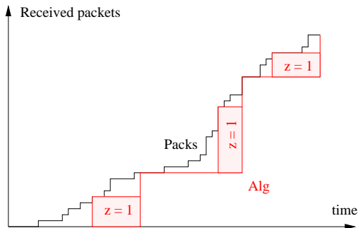
Figure 3: The z = 1 algorithm
