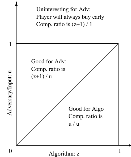
Figure 1: Choosing more than two values
