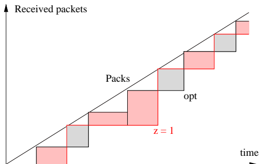
Figure 4: A_{z=1} vs. the optimal algorithm
