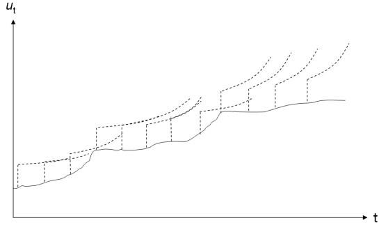
Figure 5: Visualization of \mathcal{ADV}_{nc} for the case \forall t : u_{t+1} \geq u_t . The bandwidth may increase multiplicatively in every round, but it must never exceed the constraints from previous rounds (dashed lines).
