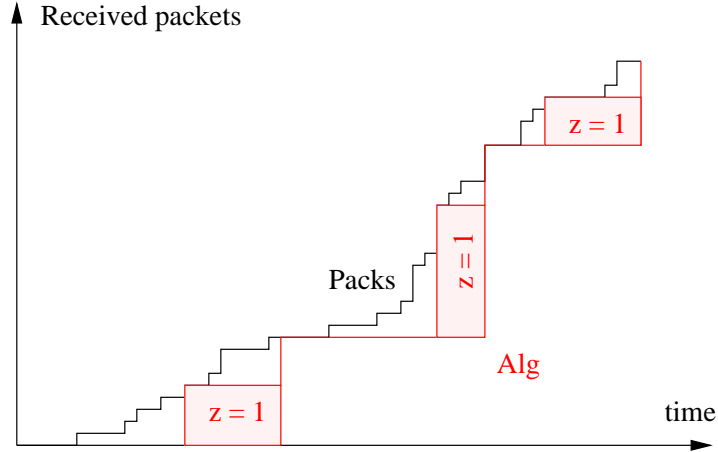
Figure 3: The z = 1 algorithm
