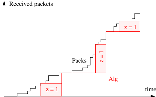
Figure 3: The z = 1 algorithm
