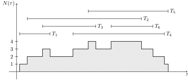
Figure 8.22: A possible realization of the random process describing a queueing system. The jobs and their response times are depicted as segments with lengths T_i , and the number of jobs in the system is given by the curve N(\tau) . In the proof of Little's Law the hatched area is measured in two ways. On the one hand, the hatched area can be obtained by taking the integral of the function N(\tau) . On the other hand, the hatched area is the sum T_1 + \dots + T_6 due to the definition of N(\tau) .
