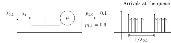
Figure 8.30: A queueing network exhibiting bursty behaviour. External jobs arrive with rate \lambda_{0,1} , and jobs leaving the queueing system immediately re-enter with probability p_{1,1} = 0.9 . Thus, in expectation, each job enters the queue 10 times before leaving the system. The external arrivals at the queue, indicated as long arrows in the right graph, are a Poisson process. However, the total arrivals at the queue are not Poisson—after serving an external arrival the job is likely to loop back to the queue a few times.
