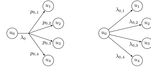
Figure 8.8: Two equivalent views: On the left, the state u_0 has a sojourn time Y exponentially distributed with parameter \lambda_0 . After time Y has passed, the next state is chosen according to the probability distribution (p_{0,1}, p_{0,2}, p_{0,3}, p_{0,4}) . On the right, the sojourn time in state 0 is \min\{Y_1, Y_2, Y_3, Y_4\} , where Y_i \sim \exp(\lambda_{0,i}) with parameter \lambda_{0,i} = p_{0,i} \cdot \lambda_0 . The next state is determined by the random variable that realizes the minimum.
