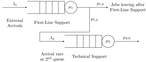
Figure 8.28: A queueing network modeling a two-tier support hotline. Jobs arrive from the outside with rate \lambda_1 and enter the queue for first-line support. After the first-line support served the job, with rate \mu_1 , a p_{1,0} = (1 - p_{1,2}) fraction of the jobs are satisfied and leave the system. The remaining p_{1,2} fraction of jobs need in-depth technical assistance, which is provided by a technician in the technical support queue. Technical support takes time exponentially distributed with parameter \mu_2 , and afterwards the job leaves the system.
