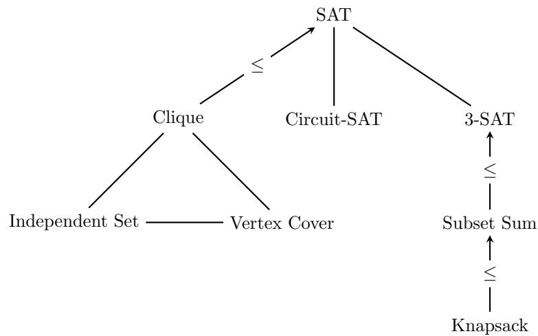
Figure 2.36: Reductions between NP-complete problems
