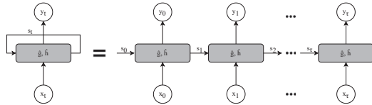
Figure 6.27: Unrolling the RNN through time. At each time step, \hat{g} and \hat{h} compute output y_t and state s_{t+1} respectively, given input x_t and the previous state s_t . BPTT propagates the gradients through the unrolled network.
