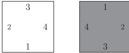
Figure 7.22: Example of a tile set consisting of two 2 tiles that tile the infinite plane in a chessboard pattern
