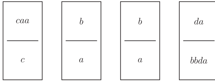
Figure 7.35: Example solution of a PCP: both the top and the bottom string is caabbda . The sequence consists of 4 dominoes, using one of the dominoes twice.
