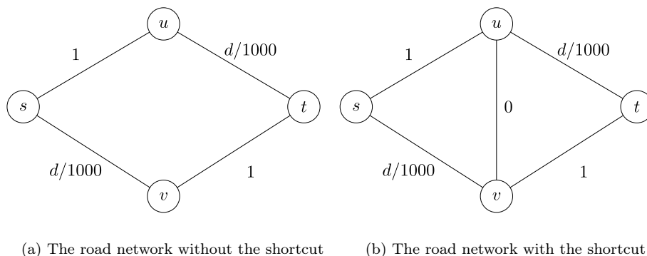
Figure 24.13: Braess' Paradox, where d denotes the number of drivers using an edge.
