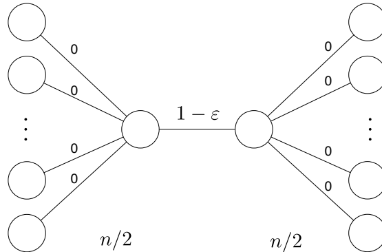
Figure 24.12: A network with a Price of Anarchy of \Theta(n) .
