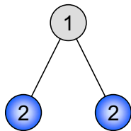
Figure 10.1: Example graph with 1) a maximal independent set (MIS) and 2) a maximum independent set (MaxIS).
